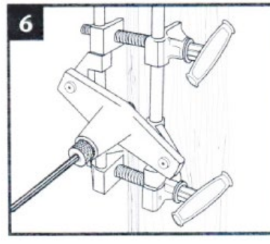
Insert drill and refit Jig to door.
